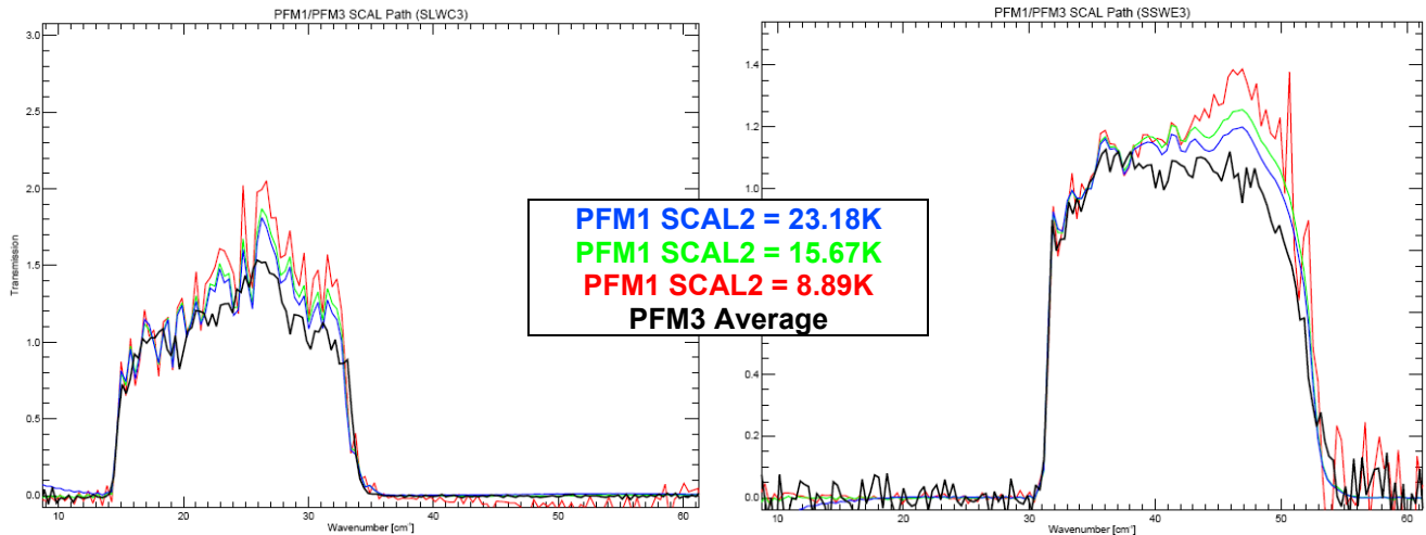
Figure 10: Comparison of the transmission for the SCAL path as derived from the PFM1 and PFM3 data. The left panel features pixel SLWC3, while the right panel shows pixel SSWE3. In each case the non-saturated transmission curves for each test campaign were averaged together.
