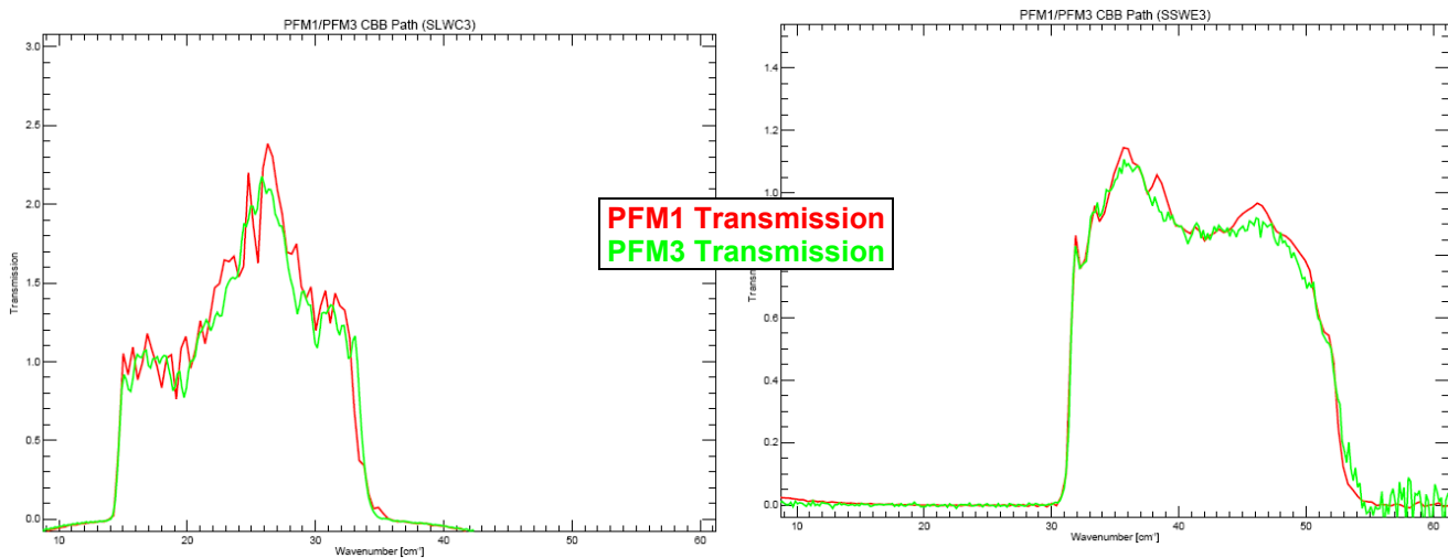
Figure 9: Comparison of the transmission for the CBB path as derived from the PFM1 and PFM3 data. The left panel features pixel SLWC3, while the right panel shows pixel SSWE3. In each case the non-saturated transmission curves for each test campaign were averaged together.
